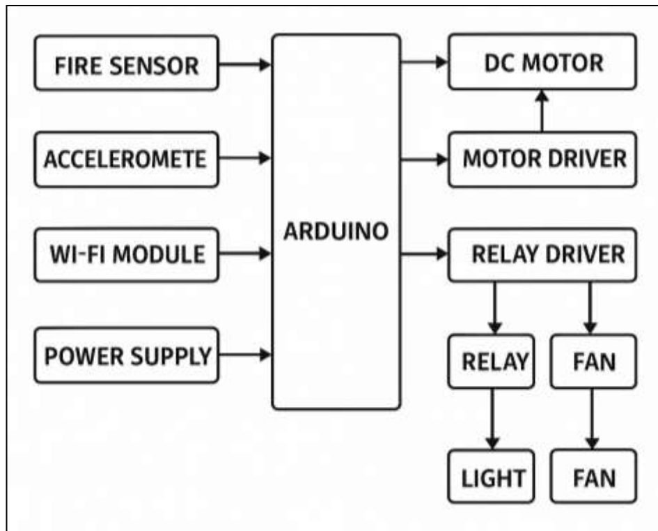
Figure1:Block Diagram of experiment
