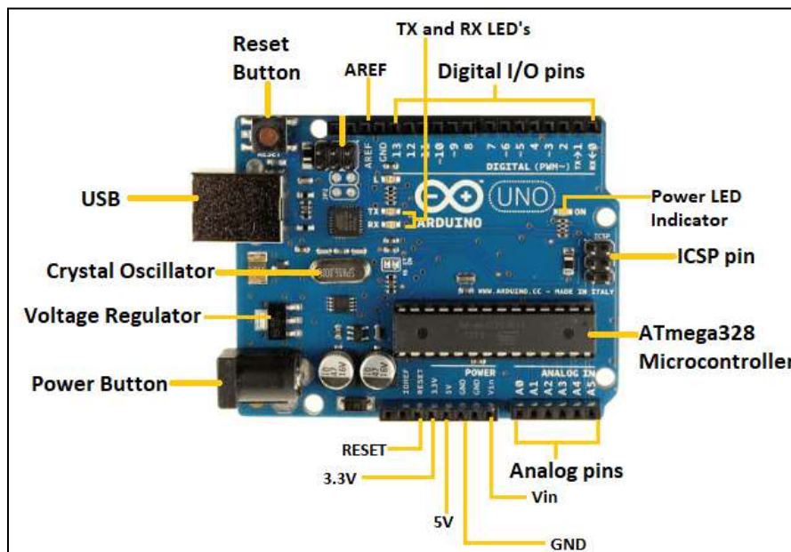
Figure2: ArduinoUNOBoard
