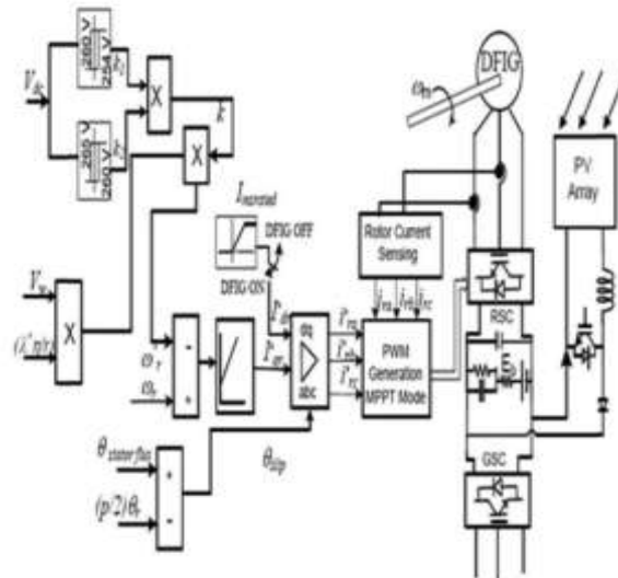
Figure 3: Control strategy of RSC
