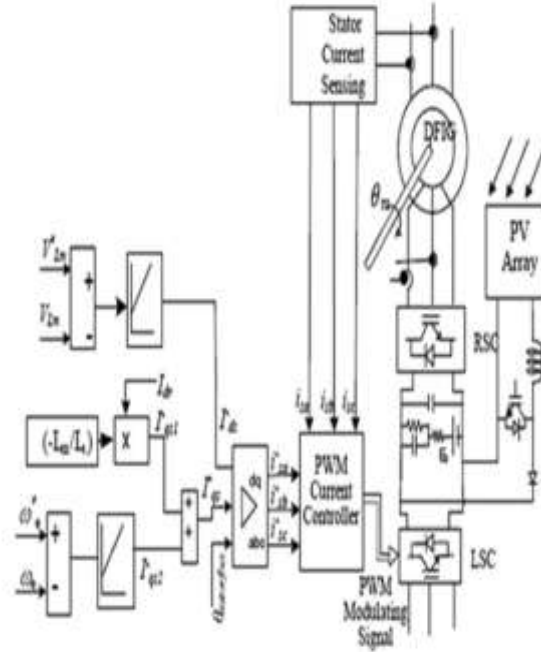
Figure 2: Control strategy of LSC
